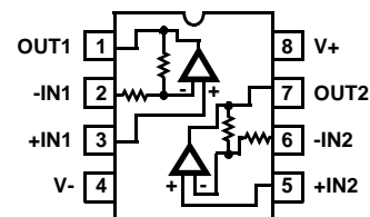
HFA1212 (SOIC) TOP VIEW
